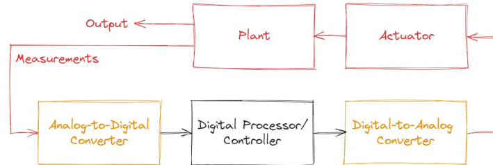
FIGURE 4.1: Block diagram of a typical digital controller system.
