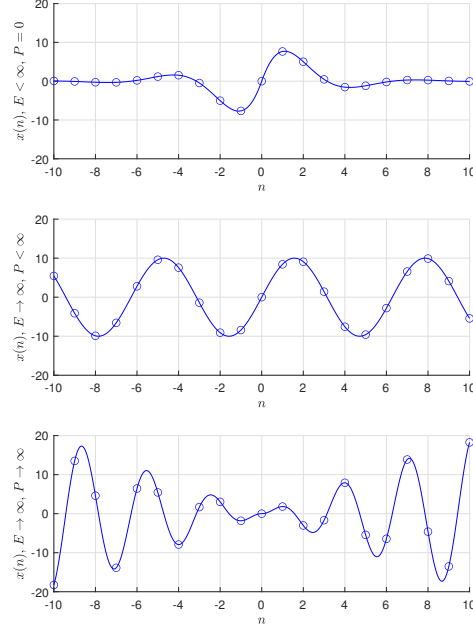
FIGURE 4.3: Example of energy and power signals, where the top plot shows an energy signal, the middle a power signal, and the bottom neither.
