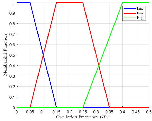
FIGURE 14.4: Membership functions for 3 fuzzy sets “low”, “fine” and “high” defined on input signal oscillation frequency.
