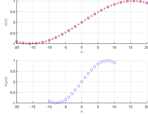
FIGURE 4.4: A demonstration of down-sampling.
