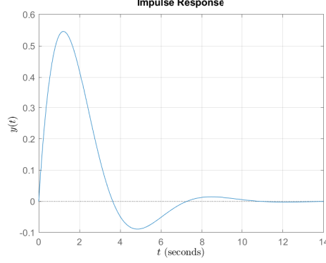
FIGURE 9.6: LTI system impulse response demonstration.
