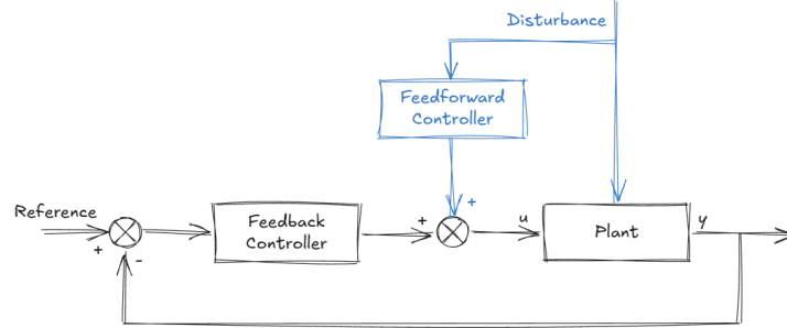
FIGURE 2.1: A closed-loop system with feedforward and feedback controllers.
