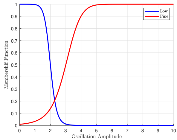
FIGURE 14.5: Membership functions for 2 fuzzy sets “low” and “fine” defined on input signal oscillation amplitude.
