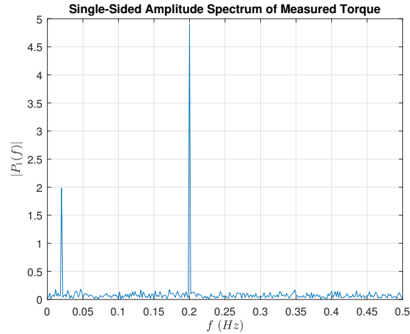
FIGURE 14.8: Measured torque single-sided amplitude spectrum.
