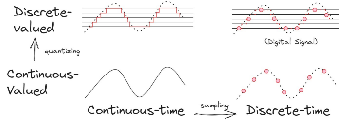
FIGURE 4.2: Continuous, discrete and digital signals.
